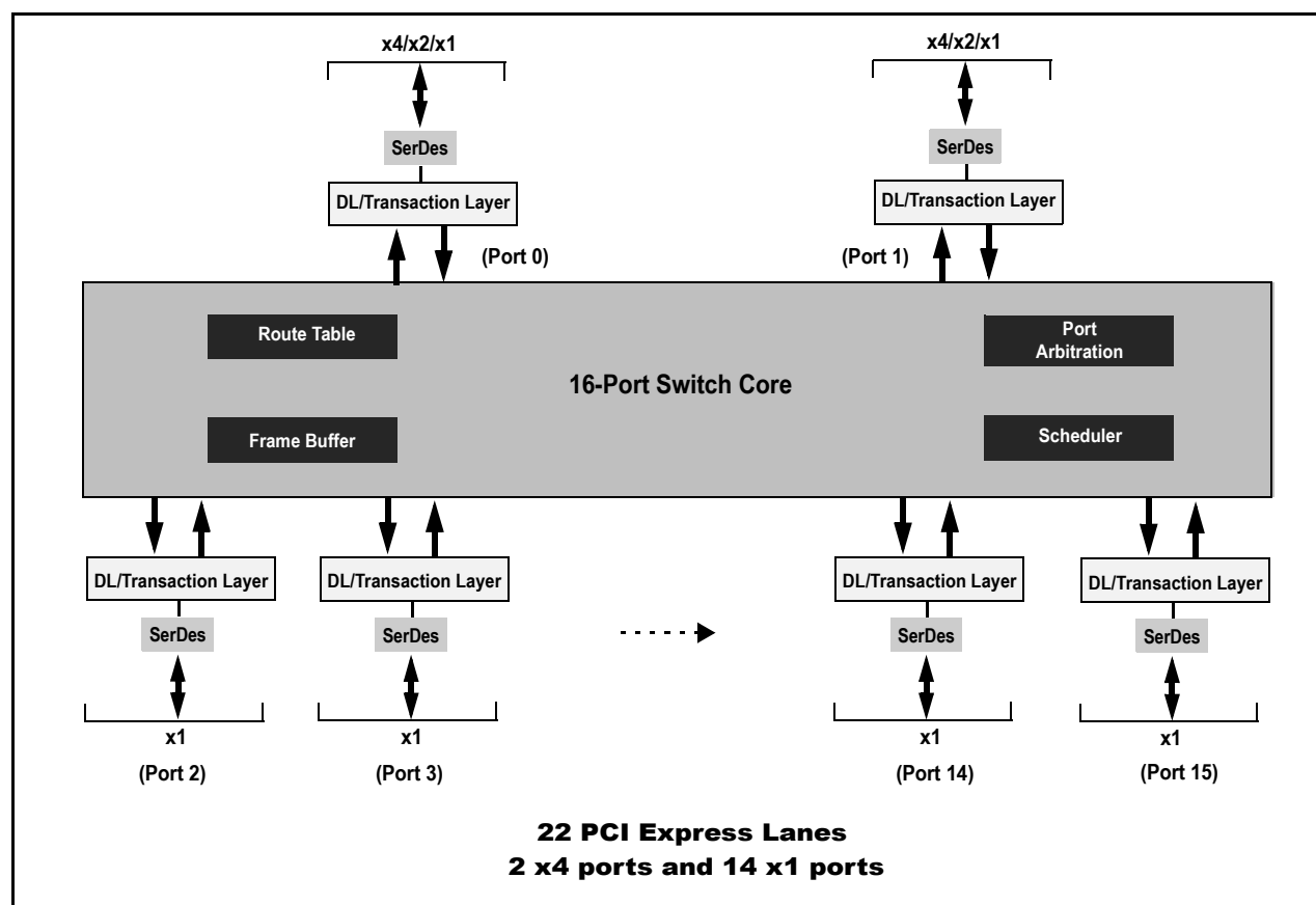
Figure 1.1 PES22H16G2 Block Diagram
