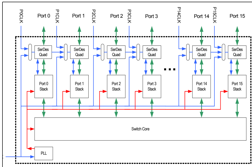
Figure 4.1 Logical Representation of the PES22H16G2 Clocking Architecture
