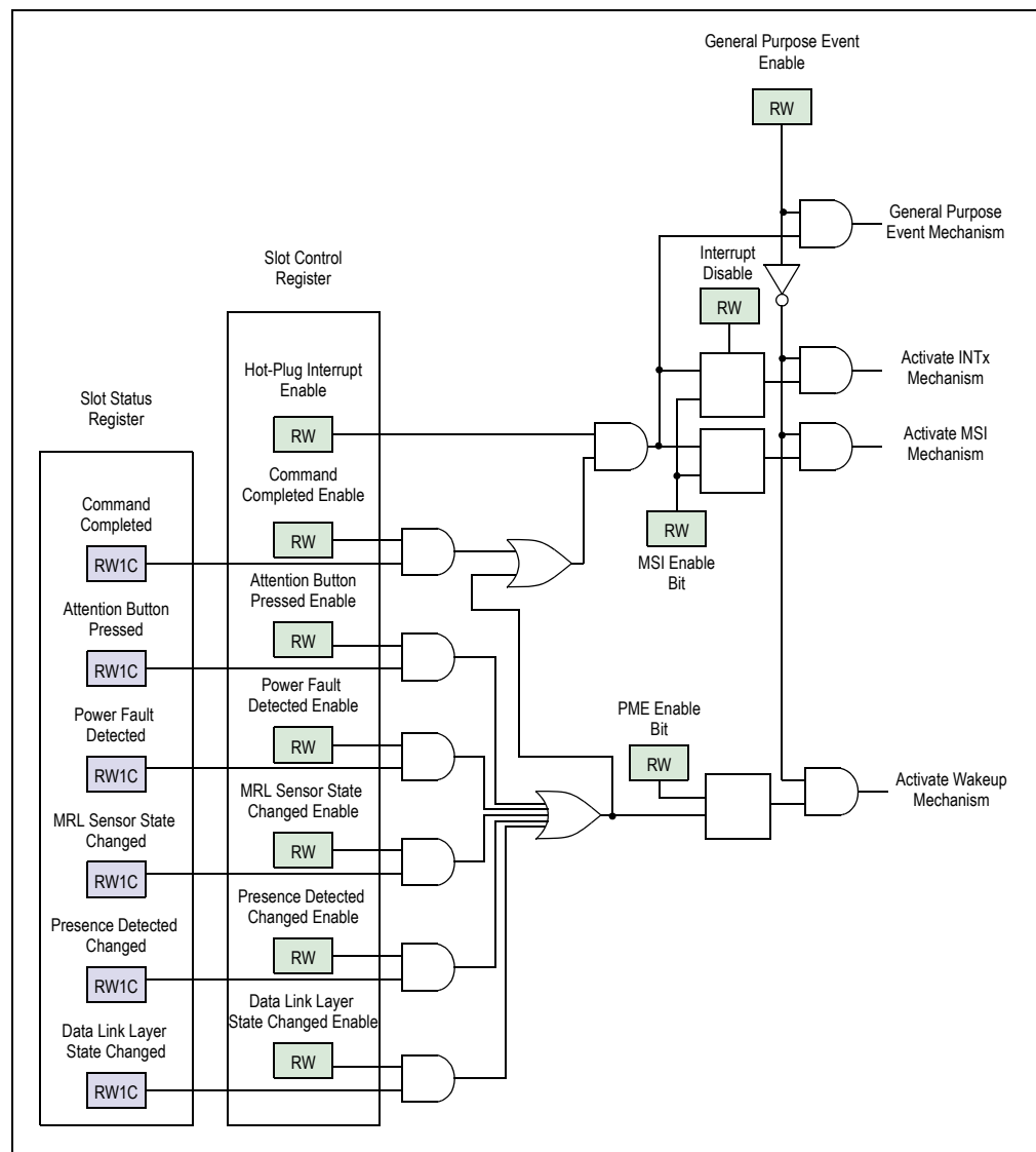
Figure 10.6 PES22H16G2 Hot-Plug Event Signalling
