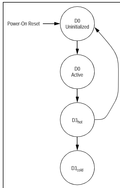
Figure 7.1 PES12N3A Power Management State Transition Diagram
