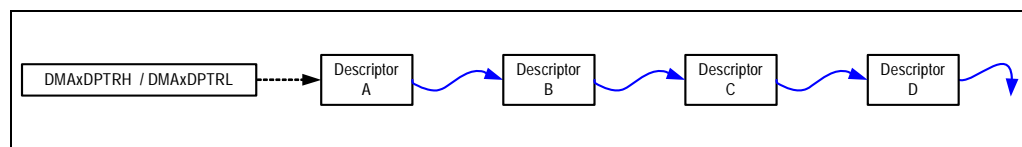
Figure 15.6 DMA Descriptor List
