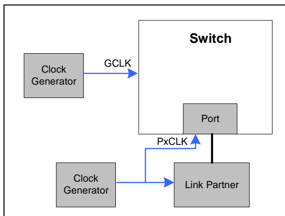
Figure 2.5 Clocking Connection for a Port in Local Port Clocked Mode, in a Common Clocked Configuration
