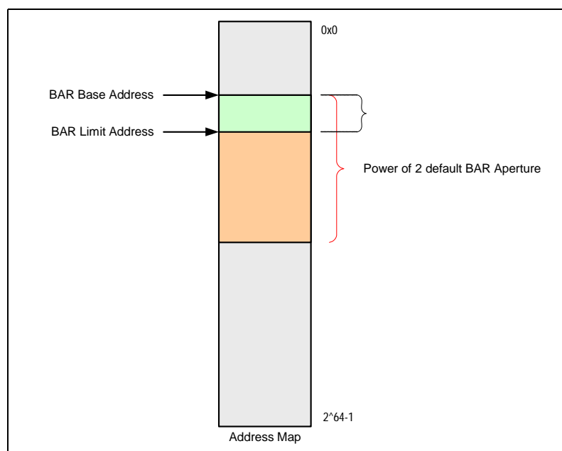
Figure 14.1 BAR Limit Operation
