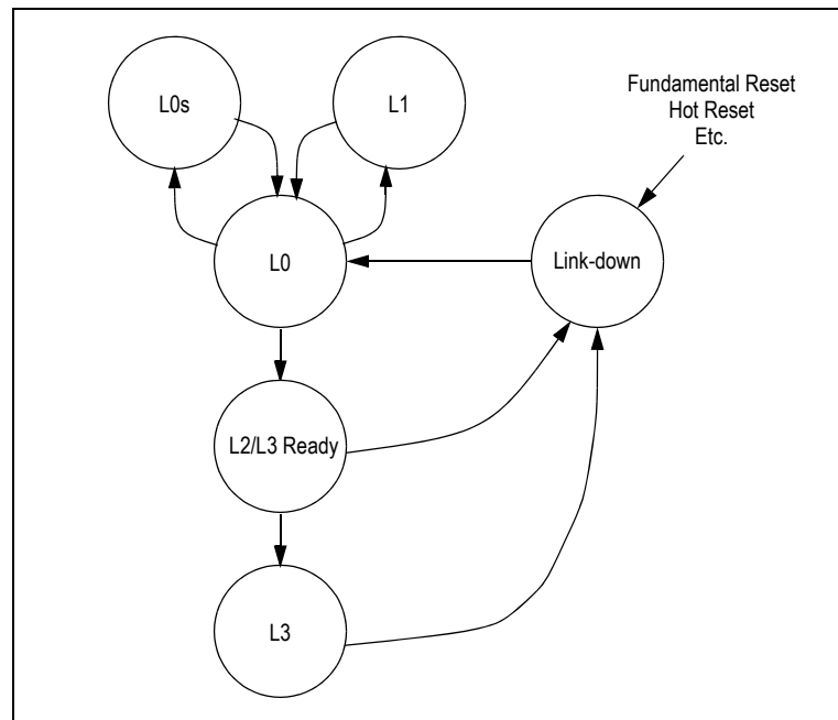
Figure 7.4 PES24NT24G2 ASPM Link State Transitions
