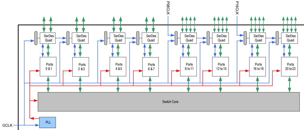
Figure 2.1 Logical Representation of PES24NT24G2 Clocking Architecture
