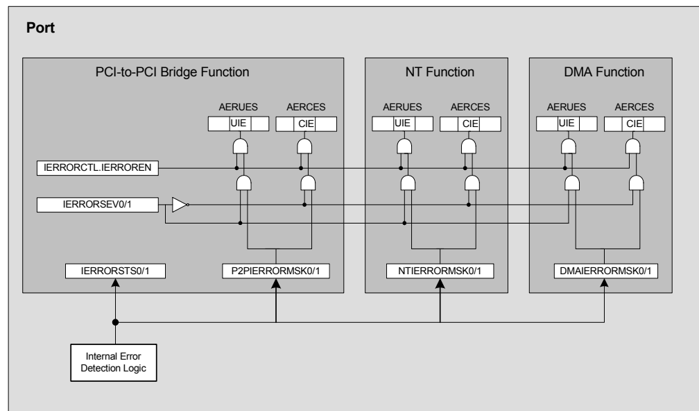
Figure 4.7 Internal Error Logic in Each PES24NT24G2 Port
