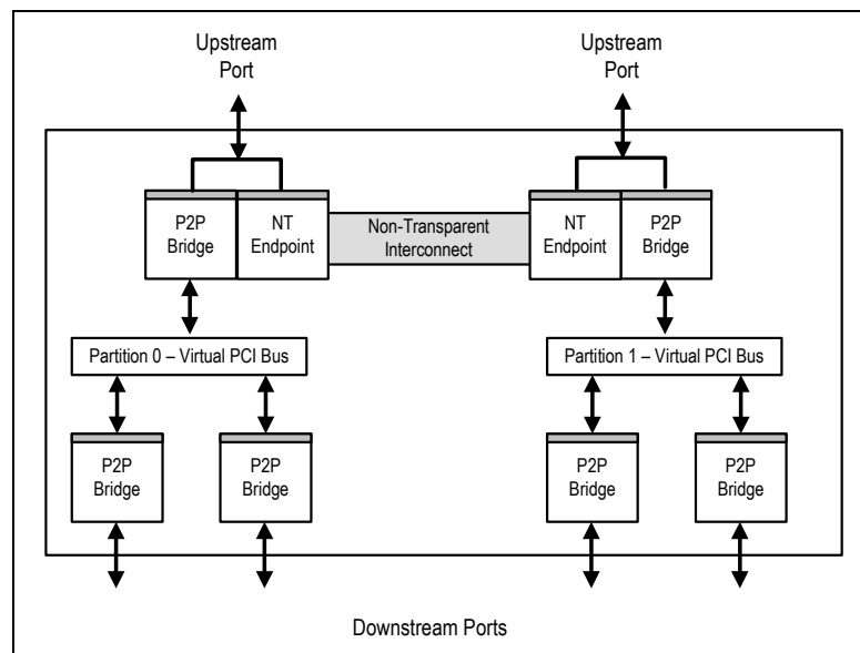
Figure 14.13 Basic Non-Transparent PES24NT24G2 Configuration
