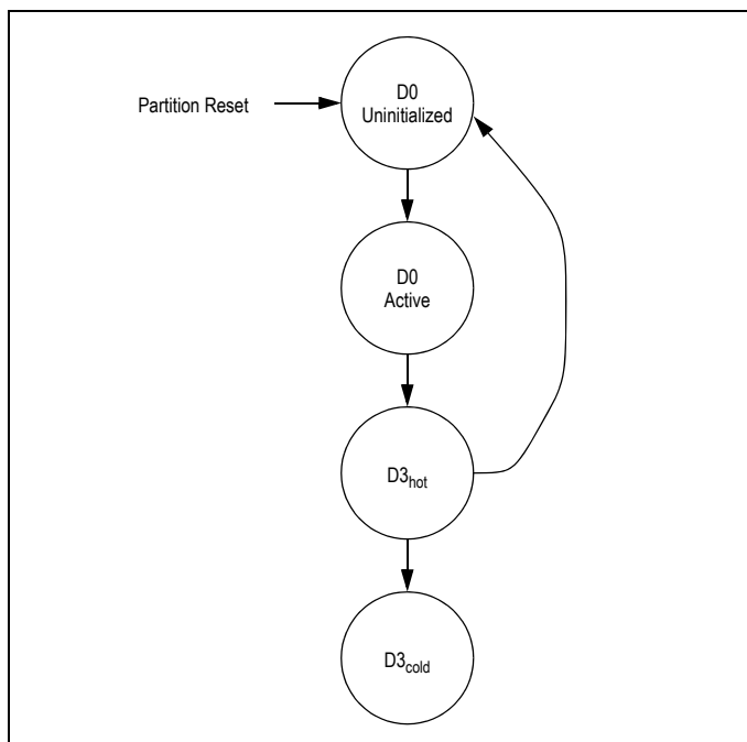
Figure 9.1 PES24NT24G2 Power Management State Transition Diagram
