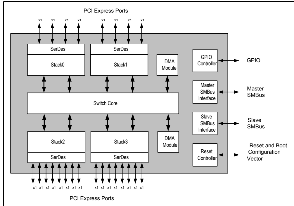
Figure 1.1 PES24NT24G2 Block Diagram
