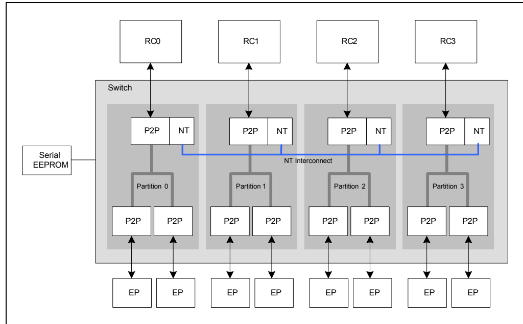
Figure 26.7 Multiprocessor System Interconnection Using the PES24NT24G2
