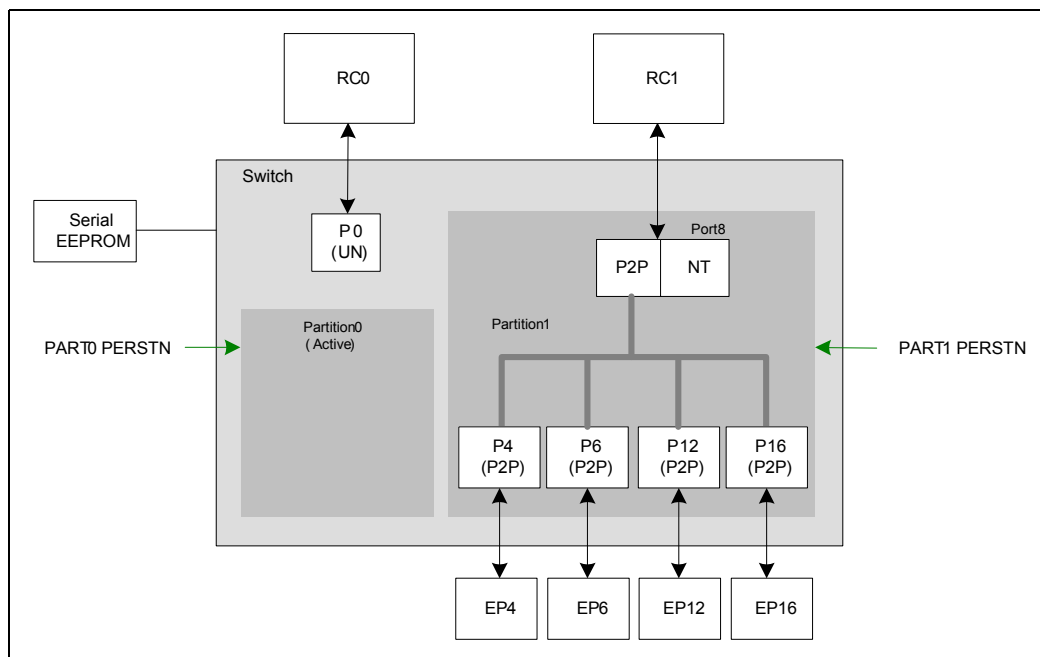
Figure 26.15 Active/Active System Configuration Before Failover Event
