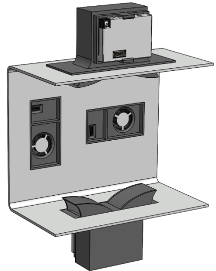
Figure 4. Design-In Examples for Air Duct
