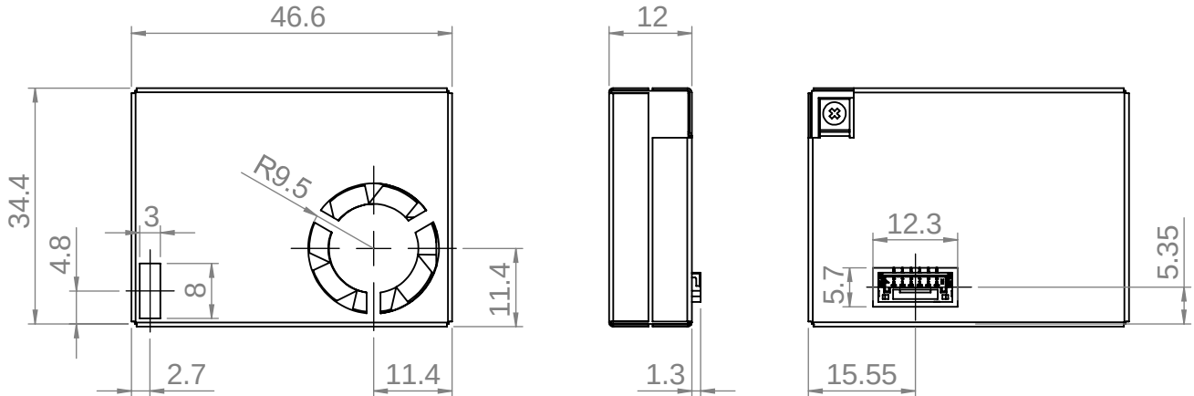
Figure 2. Package Outline Drawing (All dimensions in mm)
