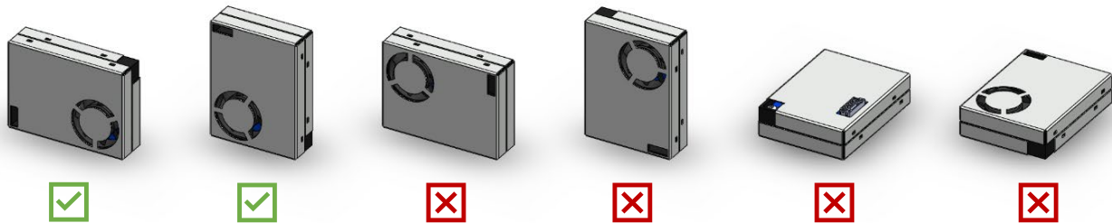
Figure 3. Recommended Orientation for Design-In
