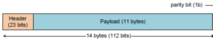
Figure 16. PWM Frame
