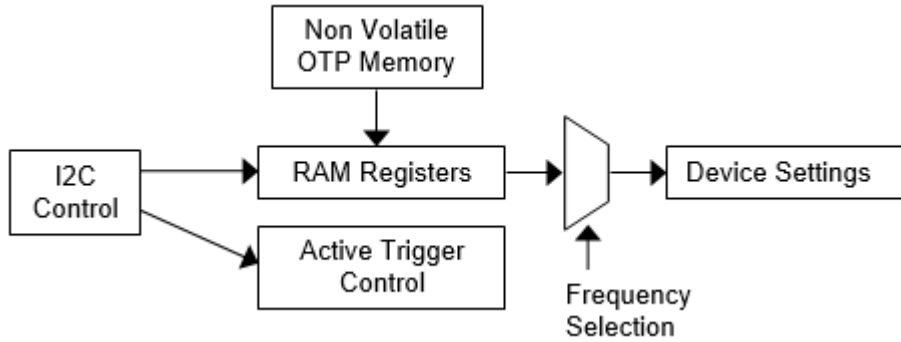
Figure 1. Register Maps
