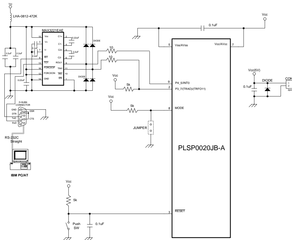
Figure 1 Connecting the Target Board to the User System
