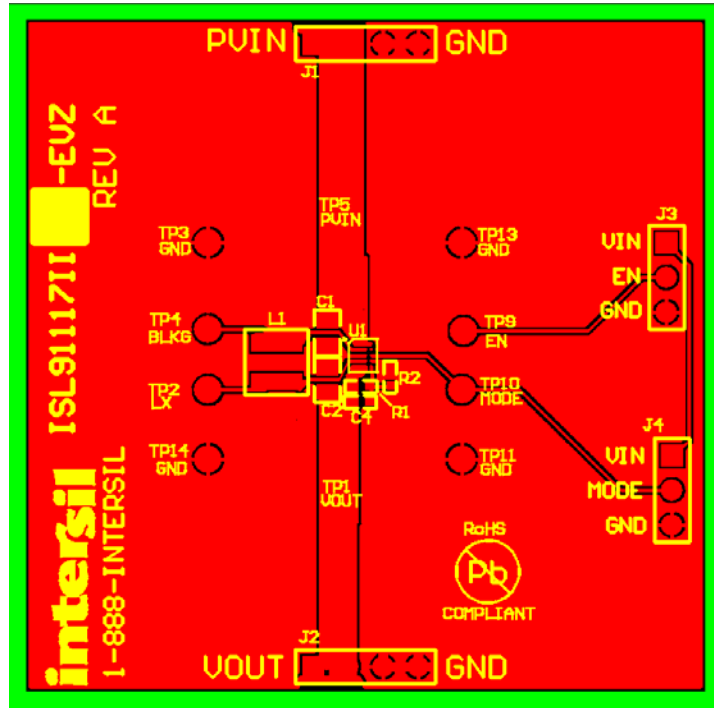
FIGURE 8. TOP LAYER
