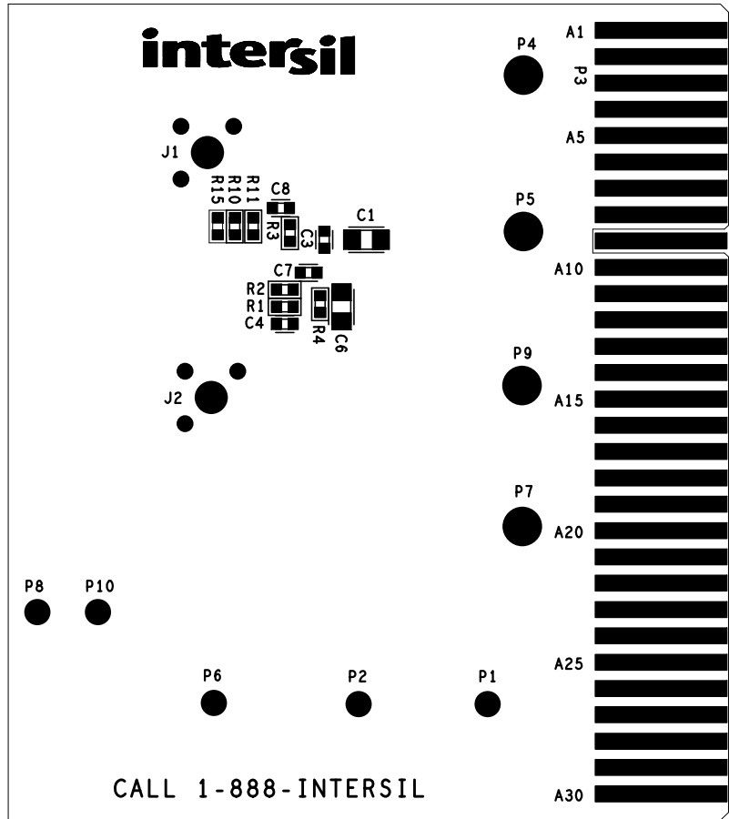
FIGURE 4. SILKSCREEN BOTTOM
