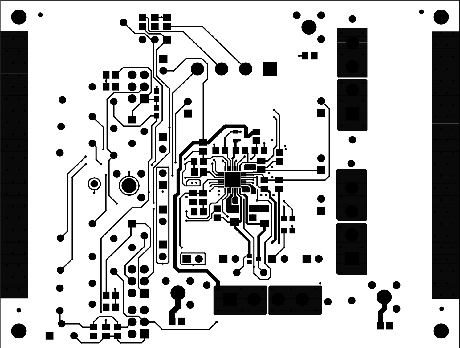
FIGURE 2. TOP LAYER
