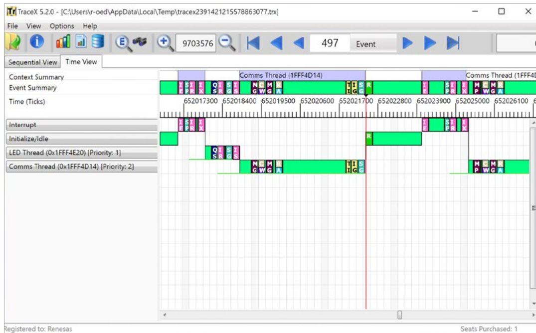
Figure 11-6: When in Time View, TraceX® displays the exact timings between the different events
