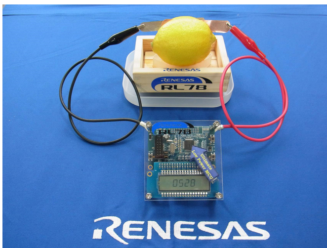
Figure 1 – Renesas RL78/L12 LCD demonstration
