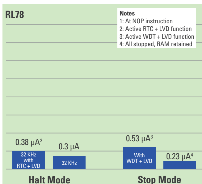
Figure 2 – RL78 Standby Current Consumption
