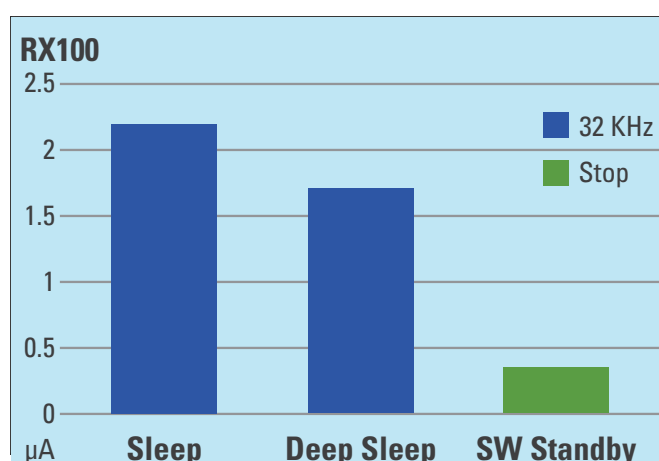
Figure 3 – RX100 Standby Current Consumption
