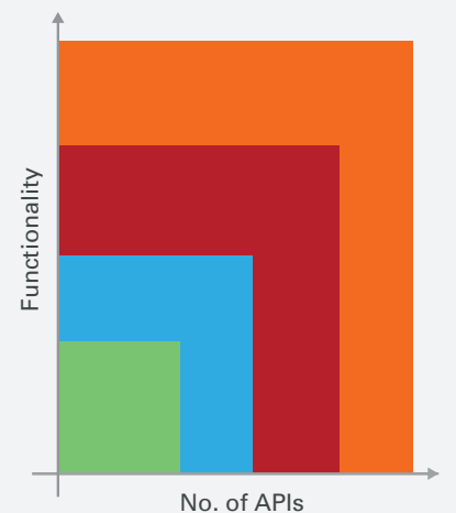
APIs & Functionality
