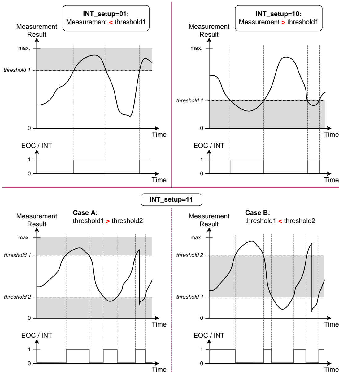
Figure 6.1 Interrupt Functionality
