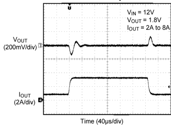
Transient Response
