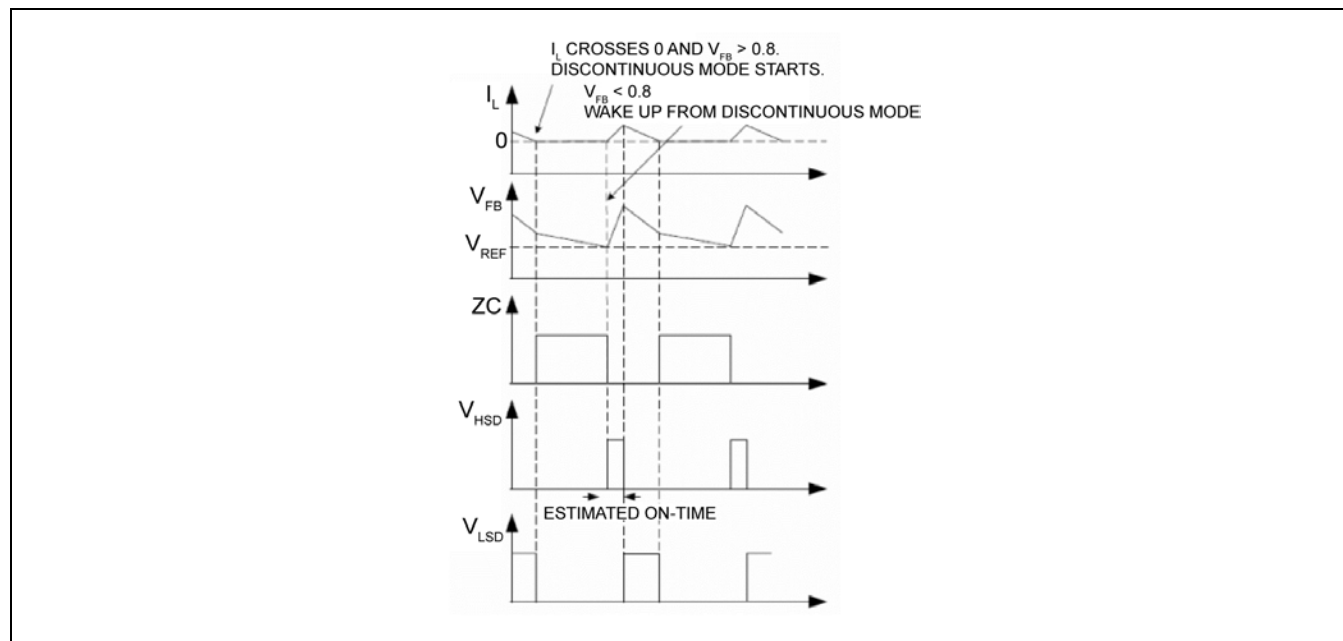
Figure 2.6 ZSPM4023-09 Control Loop Timing –Discontinuous Mode
