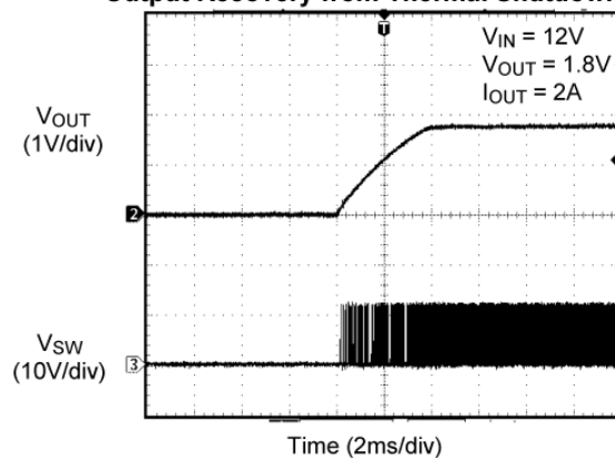
Output Recovery from Thermal Shutdown
