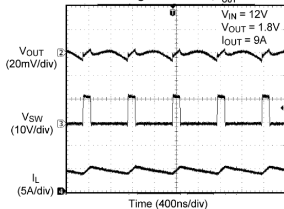
Switching Waveforms; I_{OUT} = 9A
