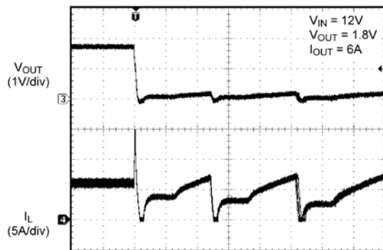
Short Circuit
