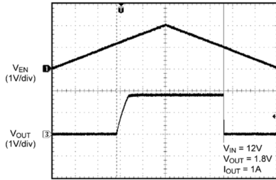
Enable Thresholds
