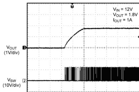
Output Recovery from Thermal Shutdown
