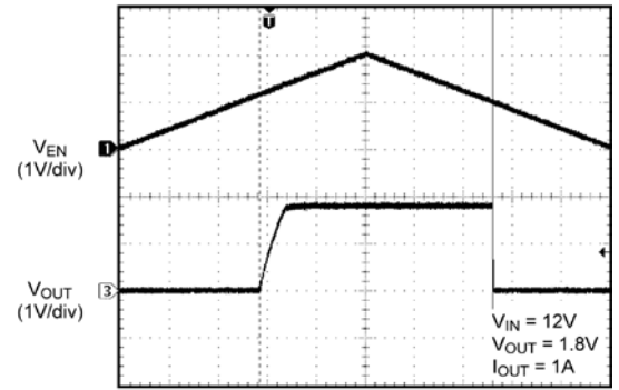
Enable Thresholds
