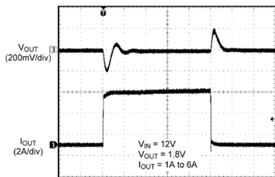
Transient Response
