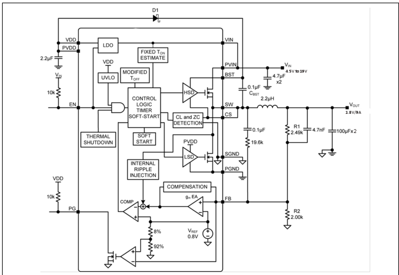
Figure 2.1 Functional Diagram
