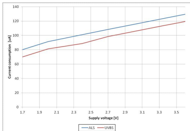
Figure 2.13 Active Current vs. Supply Voltage
