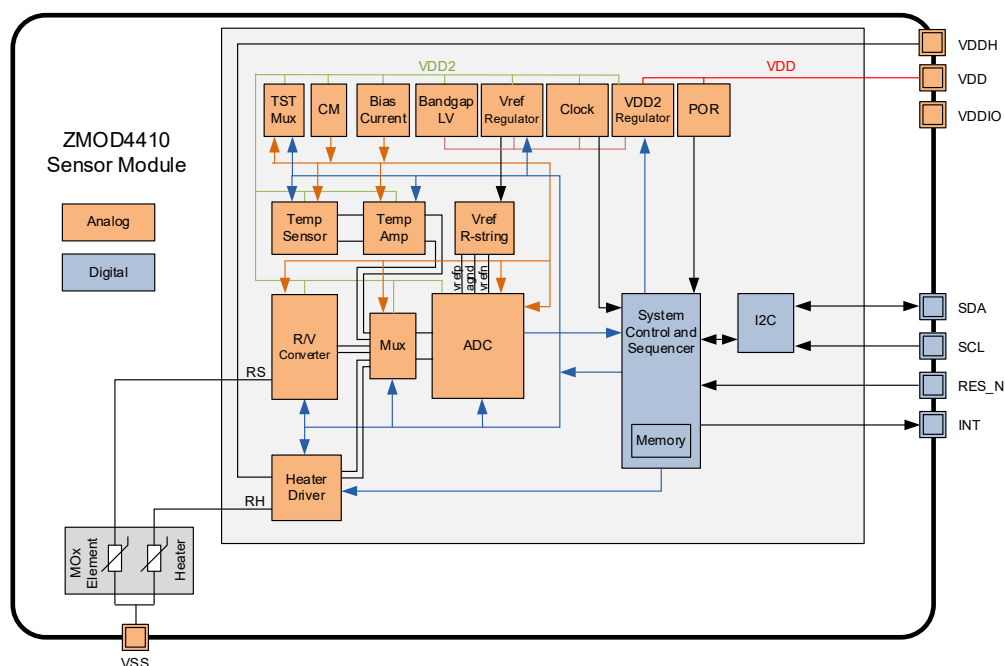
Figure 2. Block Diagram
