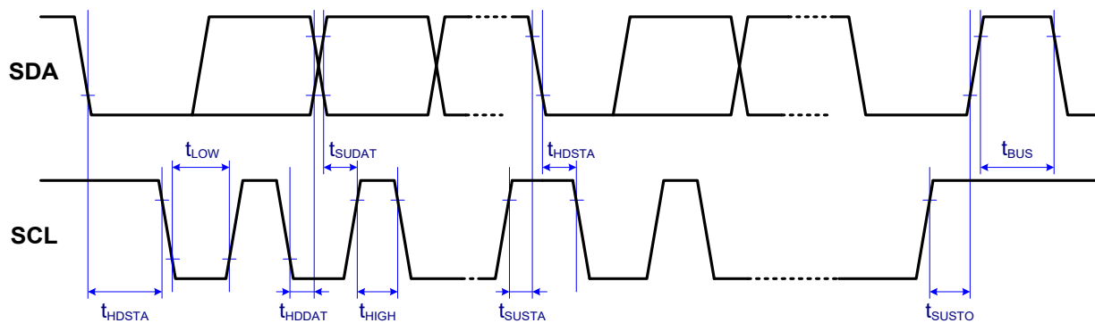
Figure 16. Bus Timing
