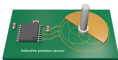
Figure 20. Example Setup: End-of-Shaft Rotation, 1 \times 360^\circ
