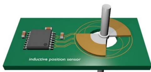
Figure 21. Example Setup: Through-Shaft Rotation, 2 \times 180^\circ
