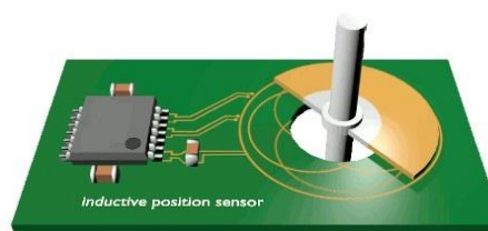
Figure 22. Example Setup: Through-Shaft Rotation, 1 \times 360^\circ
