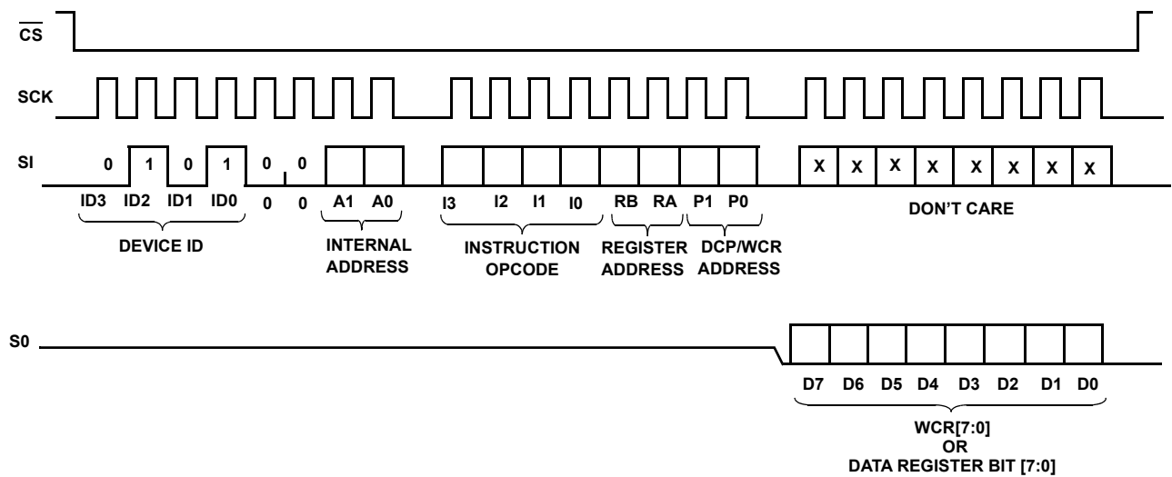
FIGURE 5. THREE-BYTE INSTRUCTION SEQUENCE SPI INTERFACE, READ CASE
