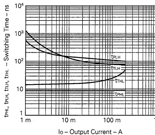
t_{PHL}, t_{PLH}, t_{THL}, t_{TLH} - I_o Characteristic
