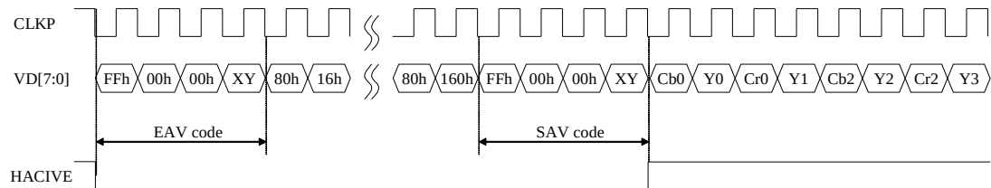
FIGURE 9. TIMING DIAGRAM OF ITU-R BT.656 FORMAT
