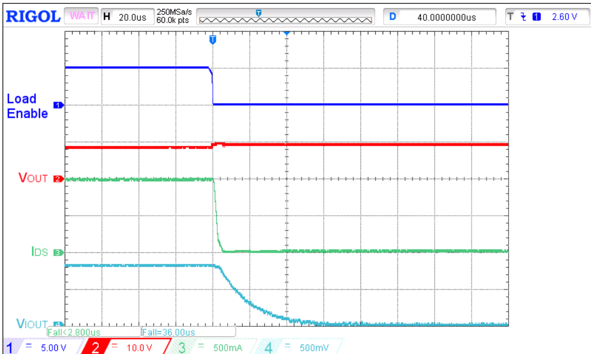
Figure 34. Typical I_{OUT} response time waveform for V_{IN} = 9 V, C_{LOAD} = 10 \mu F, R_{LOAD} = 9 \Omega , C_{IOUT} = 0.18 nF, R_{IOUT} = 84.5 k \Omega , load step 1 A to 0 A
