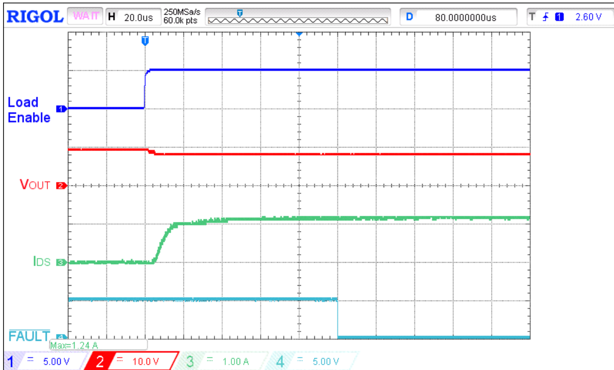
Figure 25. Typical FAULT assertion waveform for V_{IN} = 9 V, C_{LOAD} = 10 \mu F, I_{ACL} = 1 A, R_{SET} = 91 k \Omega , switch on 6.7 \Omega load
