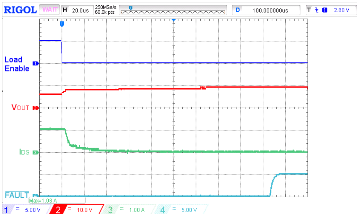
Figure 26. Typical FAULT de-assertion waveform for V_{IN} = 9 V, C_{LOAD} = 10 \mu F, I_{ACL} = 1 A, R_{SET} = 91 k \Omega , switch out 6.7 \Omega load
