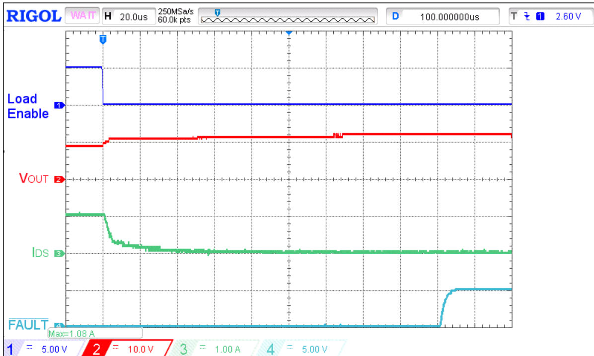
Figure 28. Typical \overline{\text{FAULT}} de-assertion waveform for V_{IN} = 12\text{ V} , C_{\text{LOAD}} = 10\text{ }\mu\text{F} , I_{\text{ACL}} = 1\text{ A} , R_{\text{SET}} = 91\text{ k}\Omega , switch out 9\text{ }\Omega load
