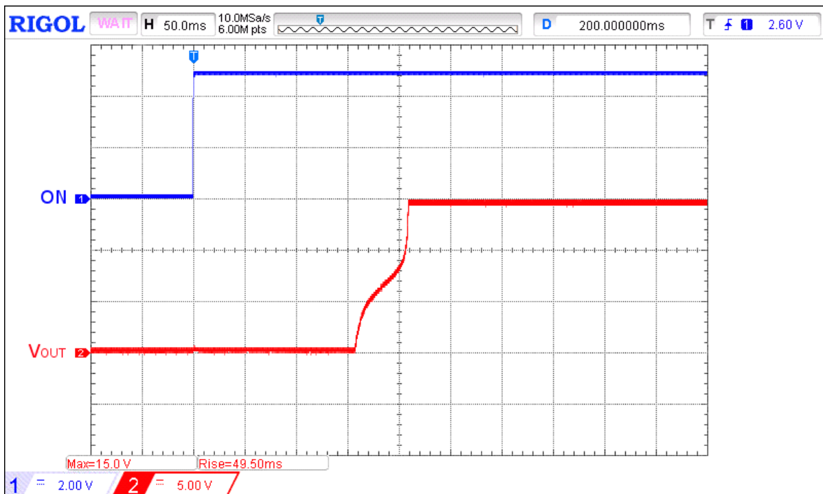
Figure 42. Typical non-monotonic V_{OUT} ramping waveform during power up on heavy load for V_{IN} = 15 V , C_{LOAD} = 470 \mu F , C_{SLEW} = 10nF , R_{SET} = 18 k\Omega , R_{LOAD} = 9.6 \Omega
