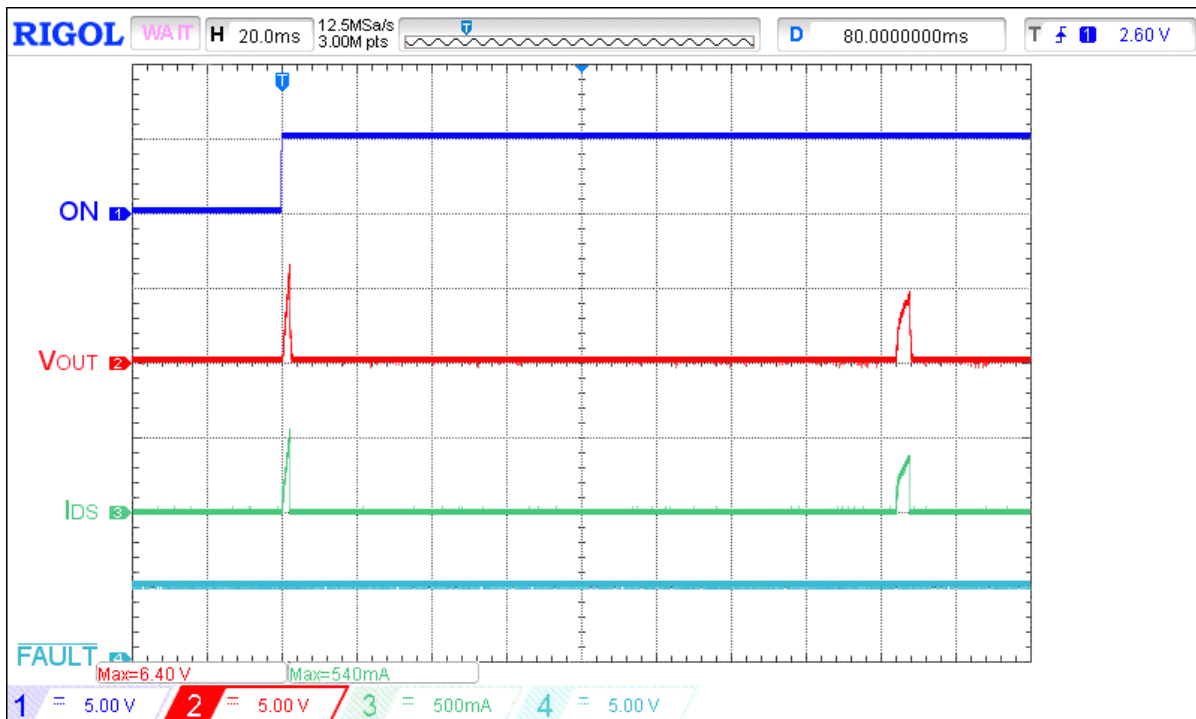
Figure 41. Extended typical SOA waveform during power up under heavy load for V_{IN} = 25.2 V , C_{LOAD} = 10 \mu F , R_{SET} = 18 k\Omega , R_{LOAD} = 12 \Omega
