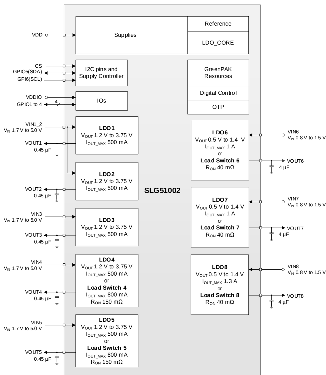
Figure 1: Block Diagram
