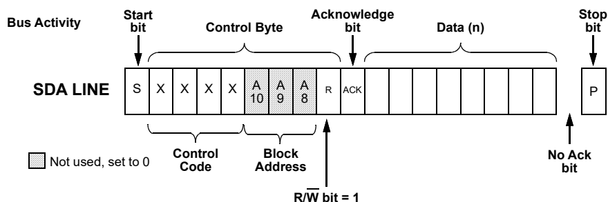
Figure 97: Current Address Read Command, \overline{R/W} = 1
