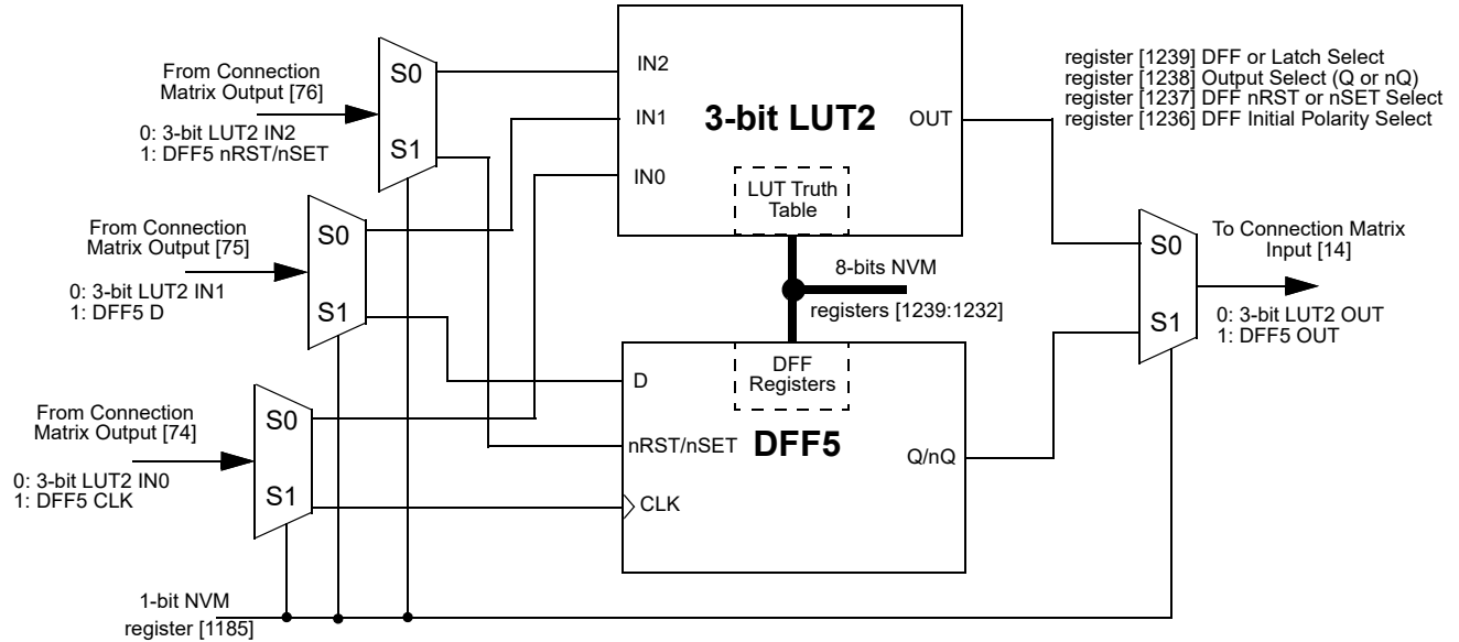
Figure 17: 3-bit LUT2 or DFF5 with RST/SET
