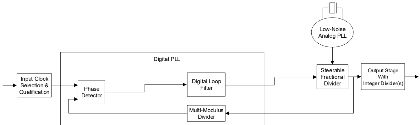
Figure 10. DPLL Channel
