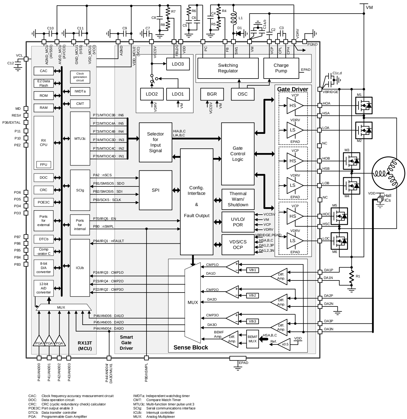
Figure 4.1-3 Simplified Block Diagram and Application – Hall Sensor Motor Drive by Using 3 Comparators
