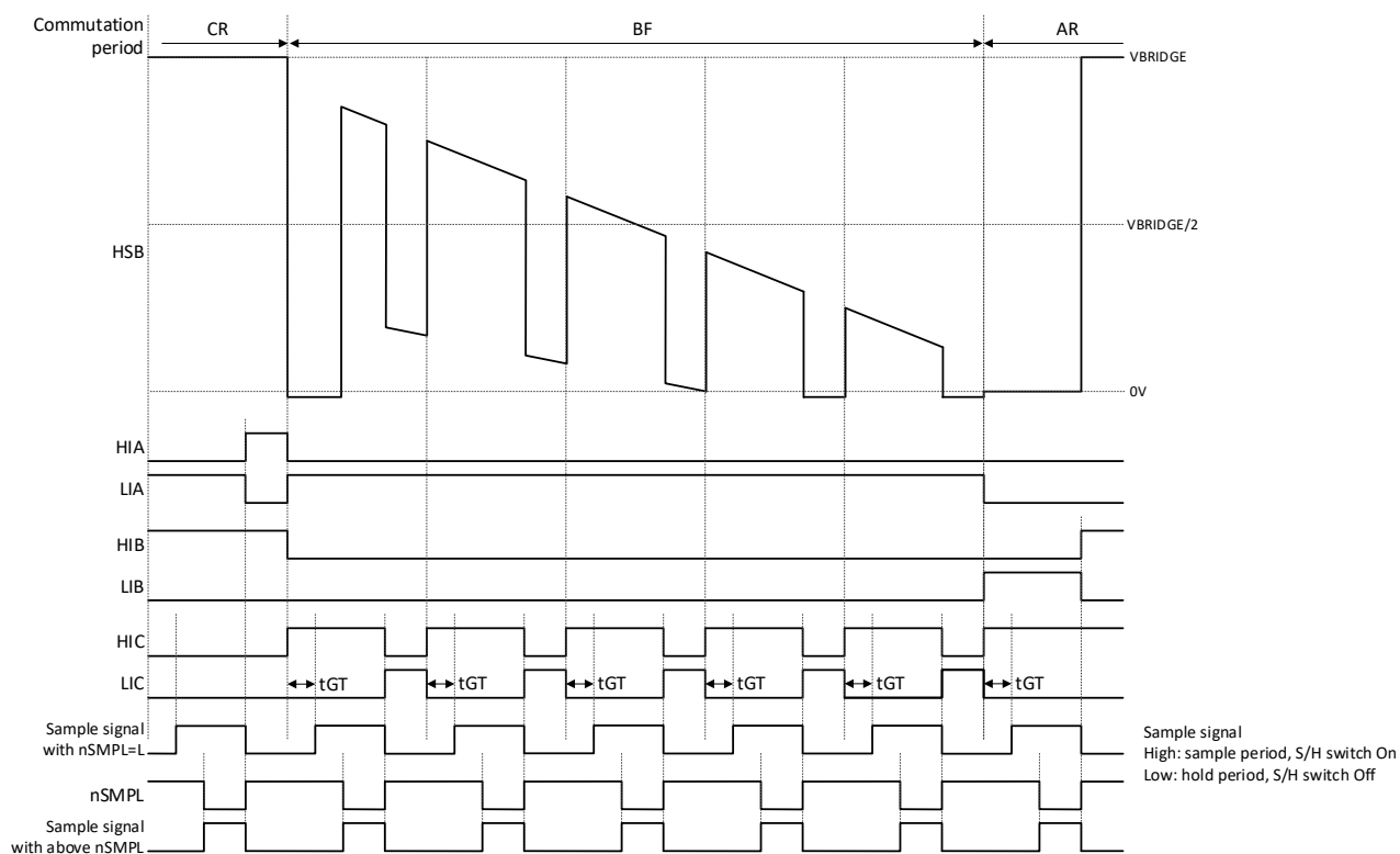
Figure 6.5-4 S/H Timing During Commutation Period BF
