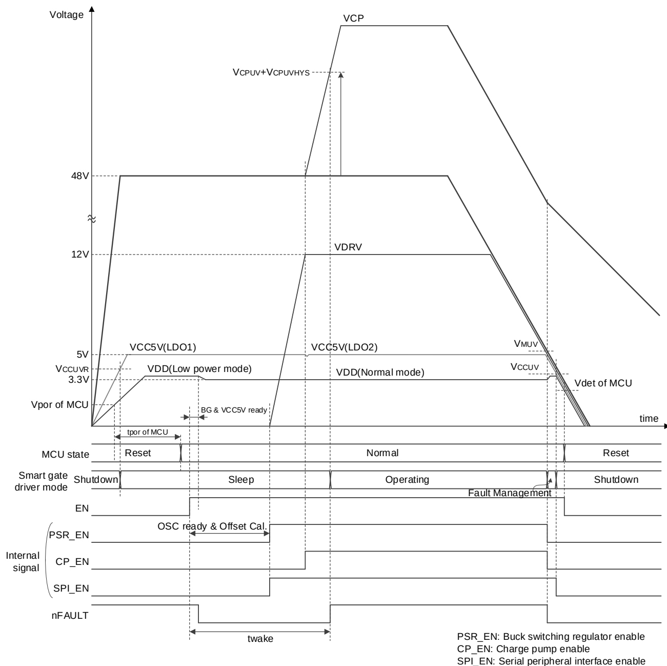
Figure 6.1-1 Power-On Sequence
