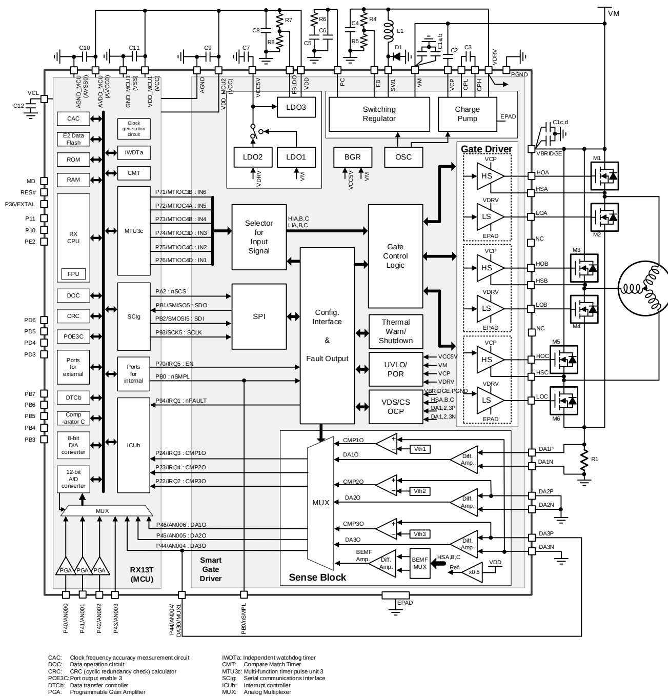
Figure 4.1-2 Simplified Block Diagram and Application – Sensorless Motor Drive by BEMF Sensing Comparator
