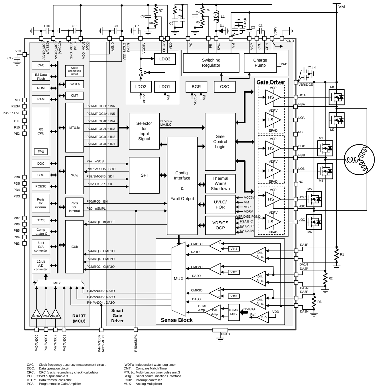
Figure 4.1-1 Simplified Block Diagram and Application – 3 Shunt Sensorless FOC Motor Drive
