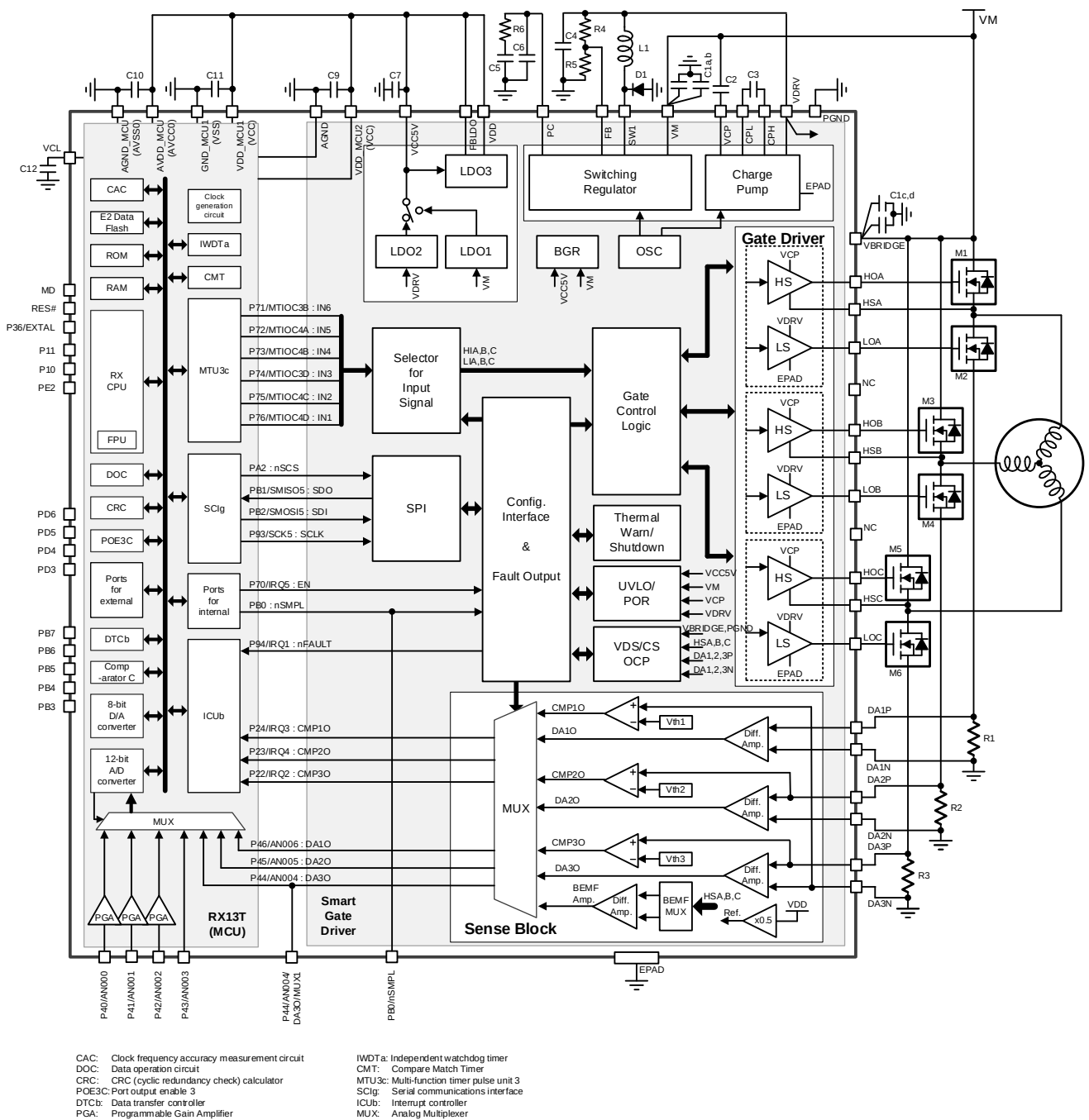
Figure 4.1-4 Simplified Block Diagram and Application – 3 Shunt Sensorless FOC Motor Drive with 5V MCU Supply
