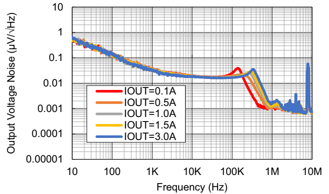
Figure 15. Output Voltage Noise for Various I_{OUT} ( V_{IN} = 3.8\text{V} , V_{OUT} = 3.3\text{V} )
