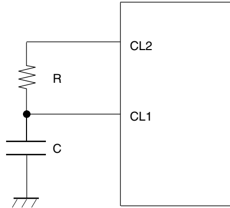
Figure 6-3: Oscillator Circuit
