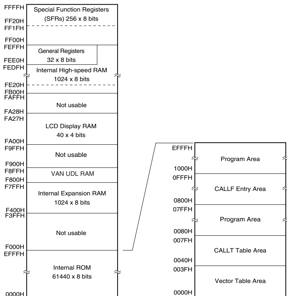
Figure 5-1: Memory Map
