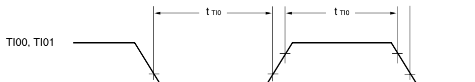
Figure 11-4: TI Timing
