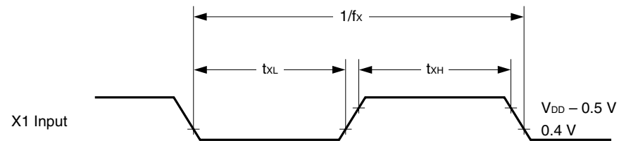
Figure 11-3: Clock Timing
