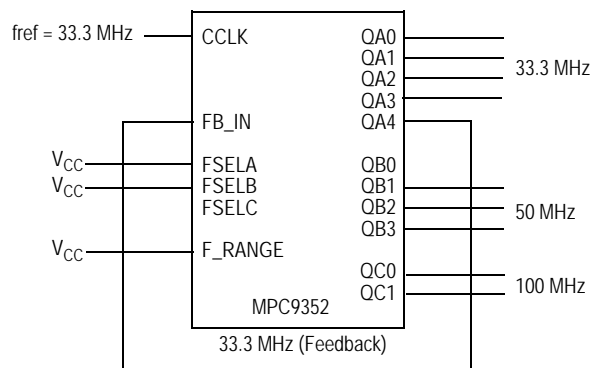
MPC9352 configuration to multiply the reference frequency by 3, 3 ÷ 2 and 1. PLL feedback of QA4 = 33.3 MHz.
