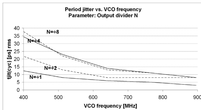
Figure 6. MPC92439 Period Jitter
