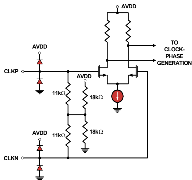
FIGURE 48. CLOCK INPUTS
