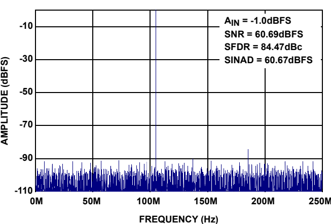
FIGURE 16. SINGLE-TONE SPECTRUM @ 105MHz
