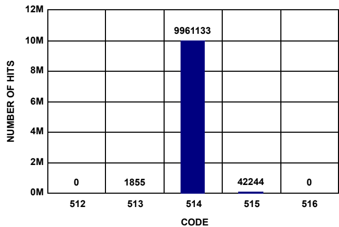
FIGURE 15. NOISE HISTOGRAM
