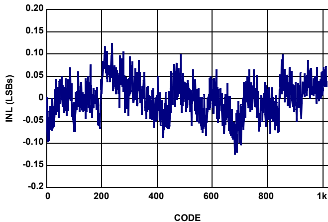
FIGURE 13. INTEGRAL NONLINEARITY
