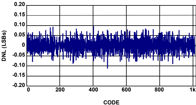
FIGURE 12. DIFFERENTIAL NONLINEARITY
