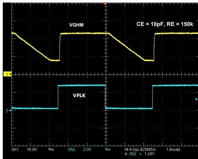
FIGURE 10. GPM CIRCUIT WAVEFORM
