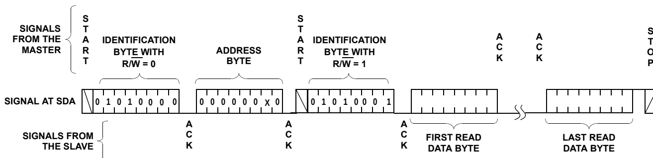
FIGURE 22. READ SEQUENCE
