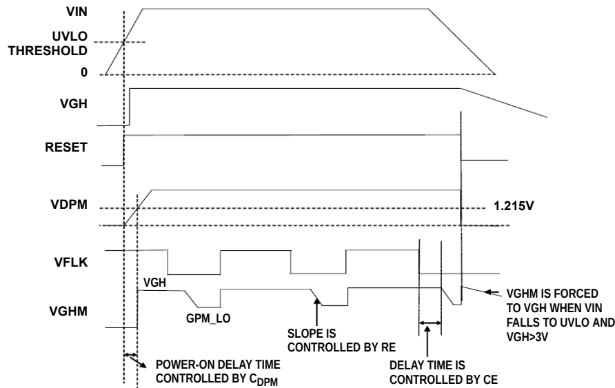
FIGURE 16. GATE PULSE MODULATOR TIMING DIAGRAM
