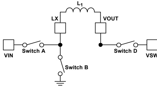
Figure 37. Buck Topology
