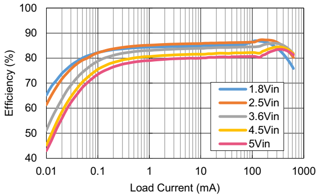
Figure 25. Efficiency vs Load Current
