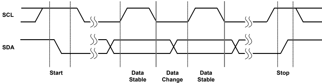
Figure 38. Valid Data Changes, Start, and Stop Conditions
