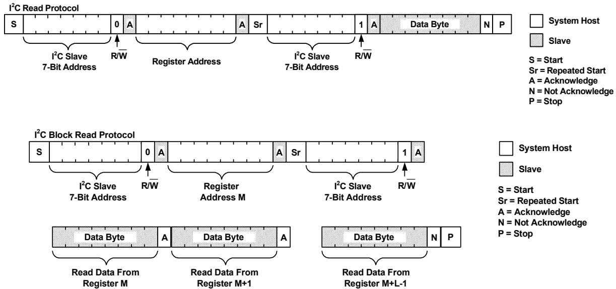
Figure 41. I 2 C Register Read Protocols
