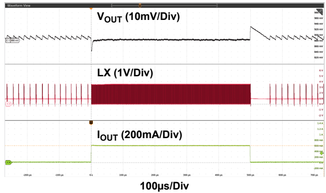
Figure 32. Load Transient: Load = 0.01A to 0.60A , Slew Rate = 1A/\mu s , Type-II Error Amplifier
