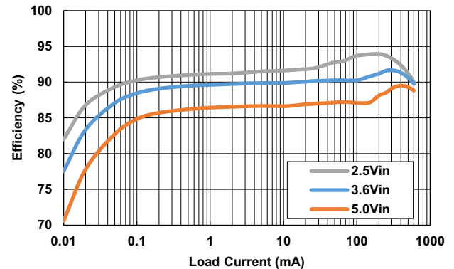
Figure 2. Efficiency vs Load Current: V_{OUT} = 1.8V , T_A = +25^\circ C (ISL9123/A)
