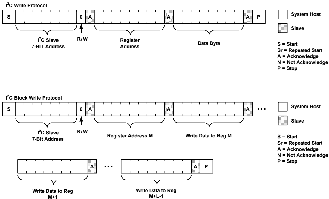
Figure 40. I2C Register Write Protocols
