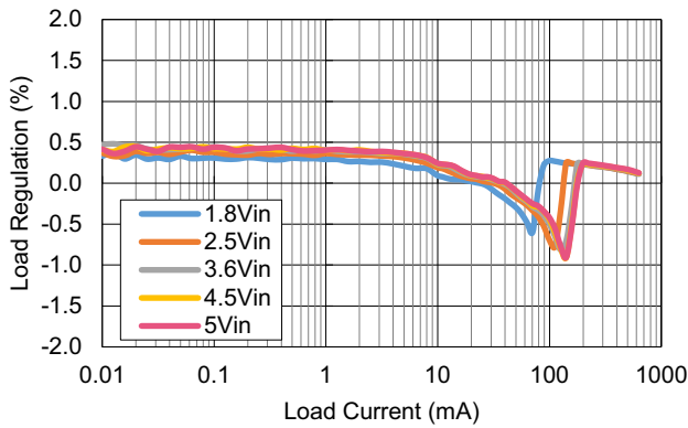
Figure 27. Output Voltage Accuracy vs Load Current
