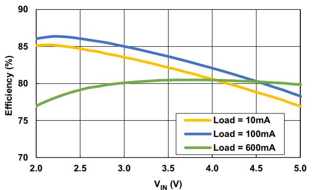
Figure 8. Efficiency vs Input Voltage: V_{OUT} = 0.8V
