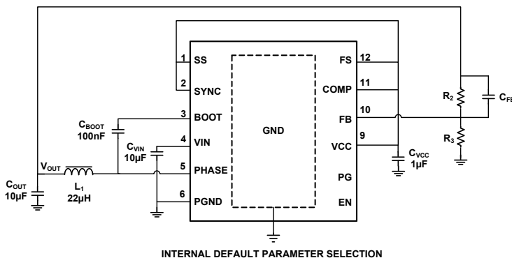
FIGURE 1. TYPICAL APPLICATION
