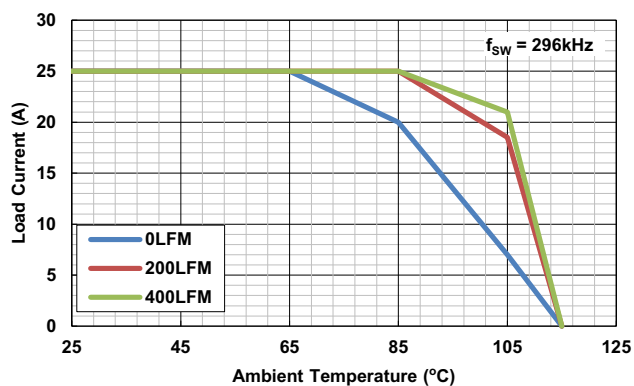
Figure 18. 5V IN to 1V OUT
