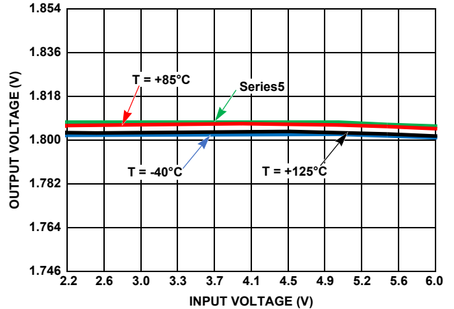
FIGURE 17. OUTPUT VOLTAGE vs INPUT VOLTAGE
