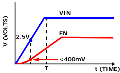
FIGURE 39. CIRCUIT IMPLEMENTATION WITH V_{IN} SLEW RATE
