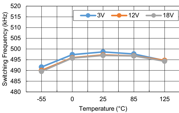
Figure 15. Switching Frequency vs Temperature
