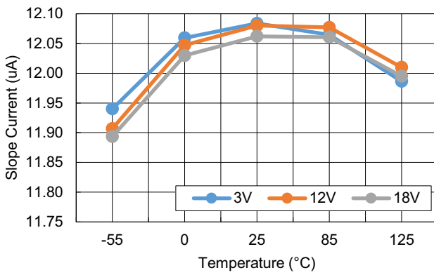
Figure 27. SLOPE Current vs Temperature
