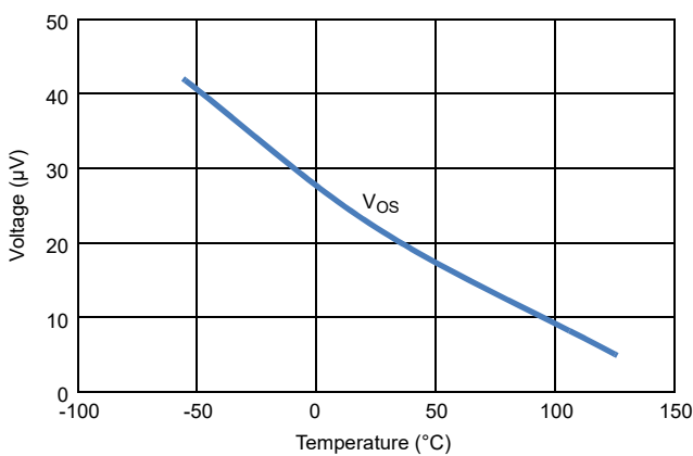
Figure 14. V_{OS} vs Temperature ( V_S = \pm 1.5V )
