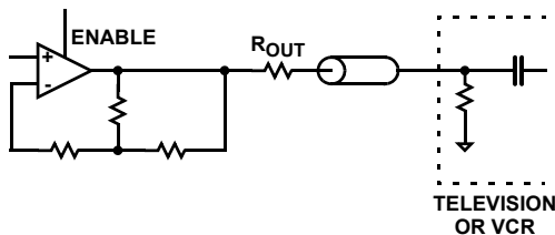
FIGURE 24. DC COUPLE
