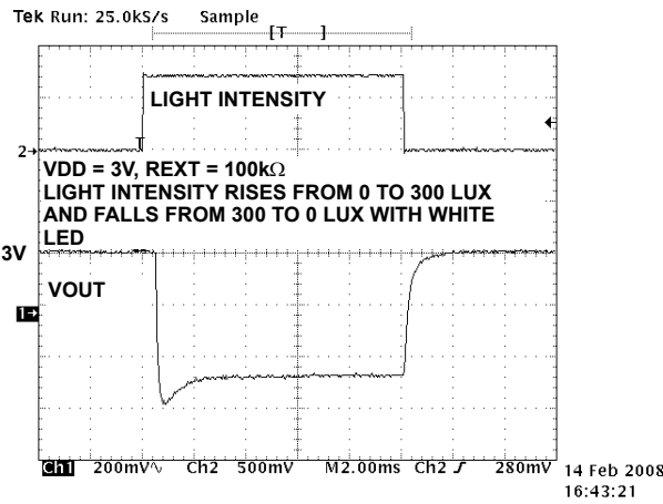
FIGURE 19. TRANSIENT RESPONSE OF ISL29007 TO CHANGE IN LIGHT INTENSITY
