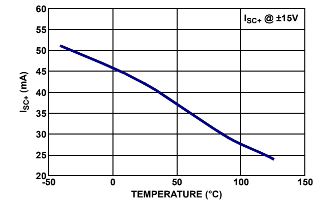
FIGURE 31. POSITIVE SHORT CIRCUIT CURRENT vs TEMPERATURE
