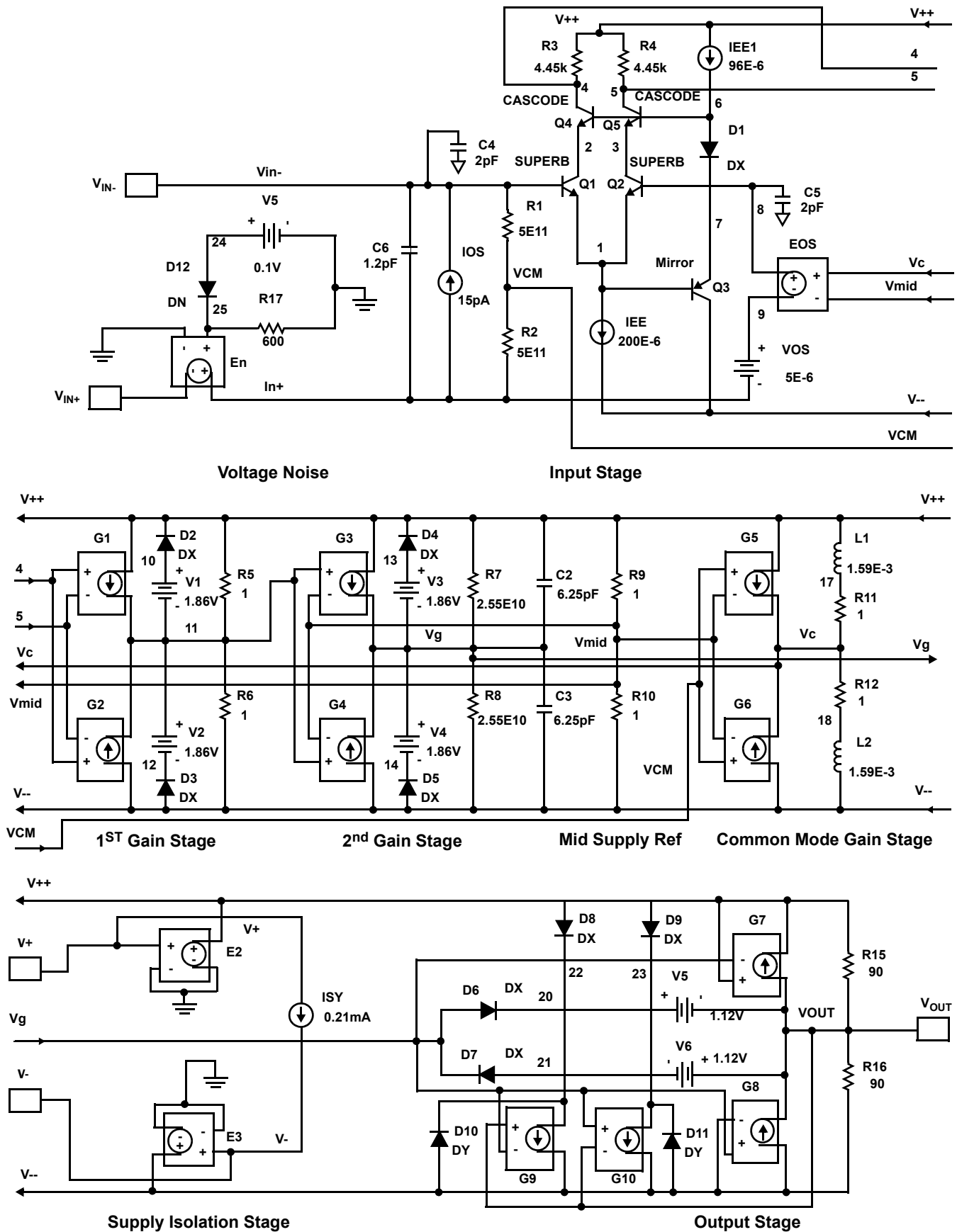
FIGURE 56. SPICE SCHEMATIC
