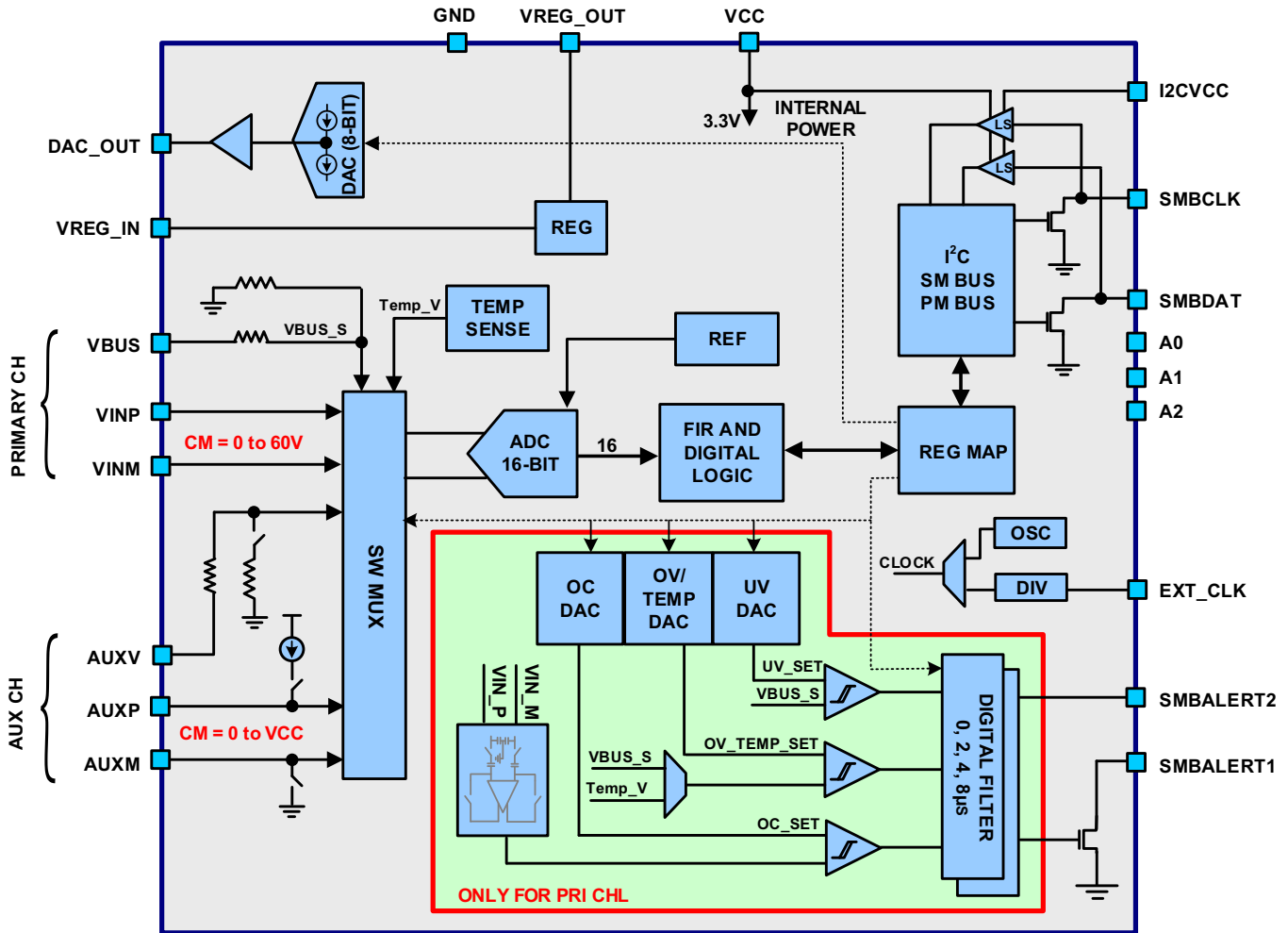
FIGURE 2. BLOCK DIAGRAM
