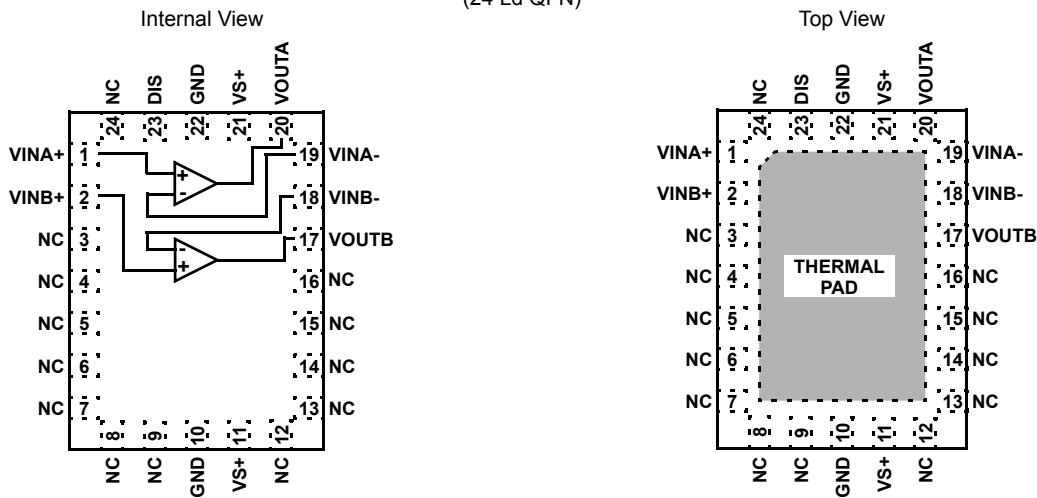
ISL15102A (24 Ld QFN)
