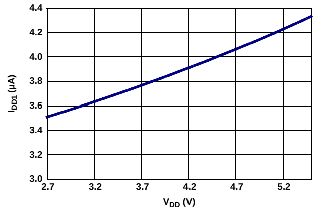
Figure 10. I_{DD1} vs V_{DD}
