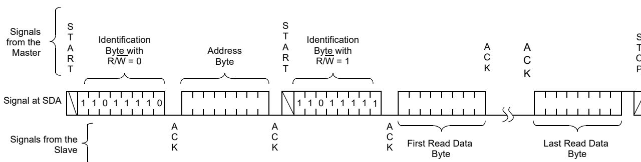
Figure 24. Read Sequence (CSR Slave Address Shown)
