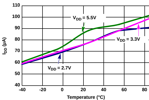
Figure 15. I_{DD} with TSE = 1 vs Temperature
