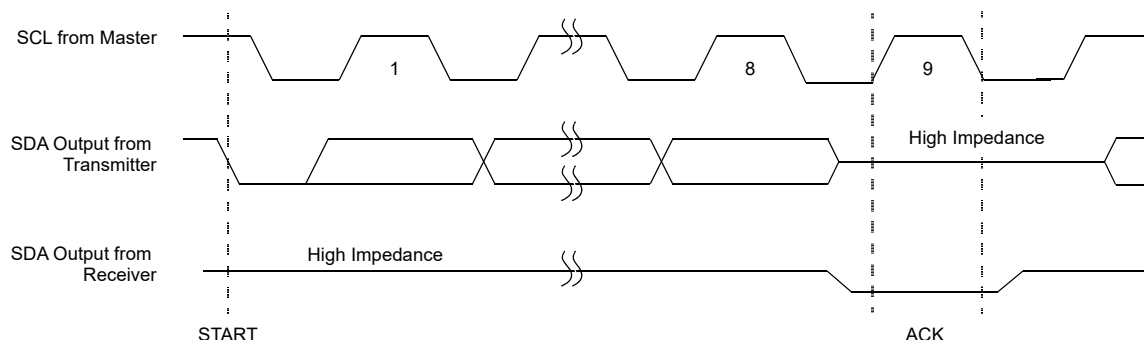
Figure 21. Acknowledge Response From Receiver
