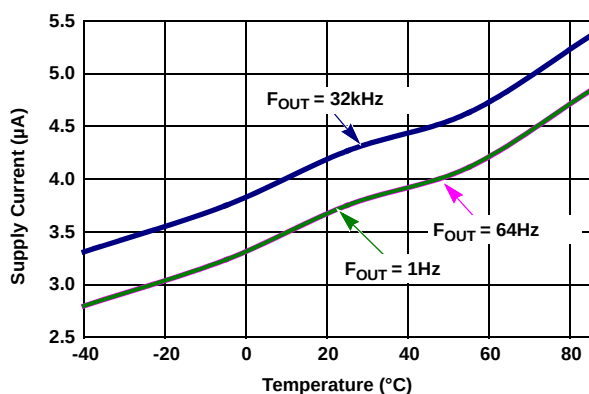
Figure 13. I_{DD} vs Temperature, 3 Different F_{OUT}
