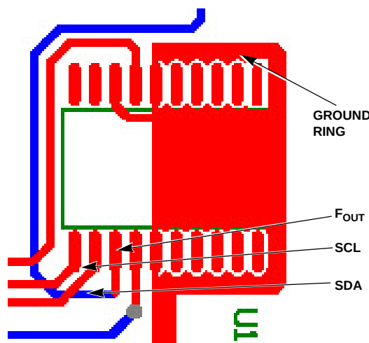
Figure 26. Suggested Layout for the ISL12022M
