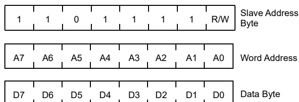
Figure 22. Slave Address, Word Address, and Data Bytes
