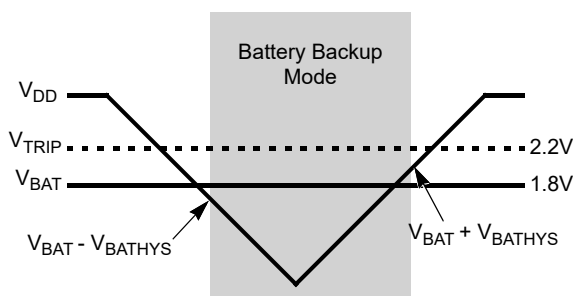
Figure 17. Battery Switchover when V_{BAT} < V_{TRIP}
