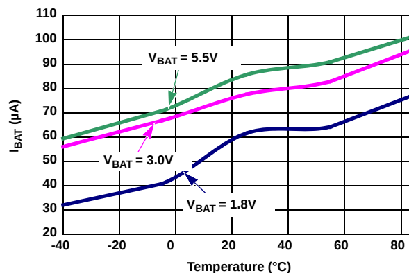
Figure 14. I_{BAT} with TSE = 1, BTSE = 1 vs Temperature
