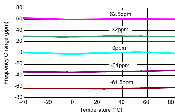
Figure 15. Oscillator Change vs Temperature at Different Aging Settings (IATR) (BETA Set for 1ppm Steps)
