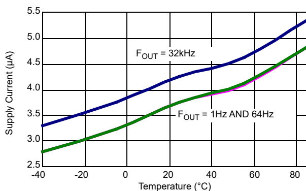
Figure 12. I_{DD} vs Temperature, 3 Different F_{OUT}
