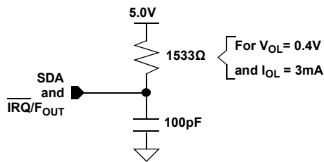
Figure 4. Standard Output Load for Testing the Device with V_{DD} = 5.0V
