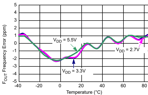
Figure 10. Oscillator Error vs Temperature
