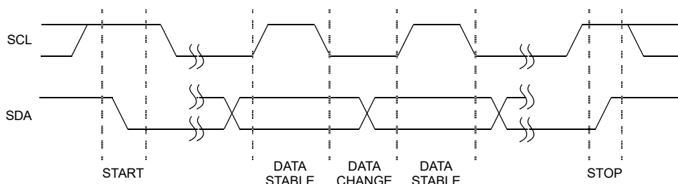
Figure 19. Valid Data Changes, Start and Stop Conditions
