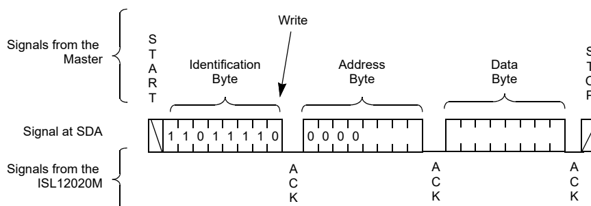
Figure 22. Byte Write Sequence (Slave Address for CSR Shown)
