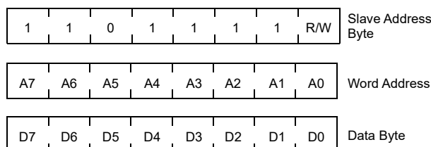
Figure 21. Slave Address, Word Address, and Data Bytes
