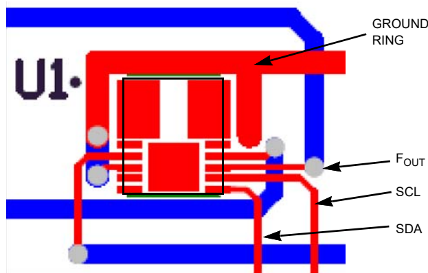
Figure 25. Suggested Layout for ISL12020M
