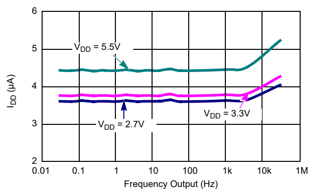
Figure 11. F_{OUT} vs I_{DD}
