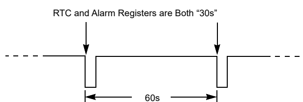
Figure 18. \overline{\text{IRQ}}/\text{F}_{\text{OUT}} Waveform
