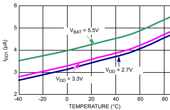
Figure 8. I_{DD1} vs Temperature
