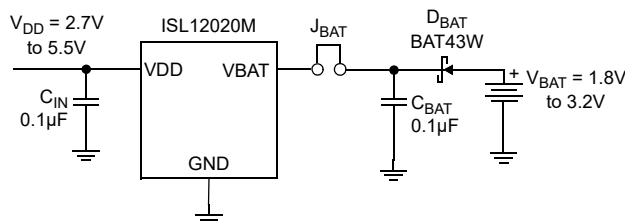
Figure 24. Suggested Battery-Backup Circuit
