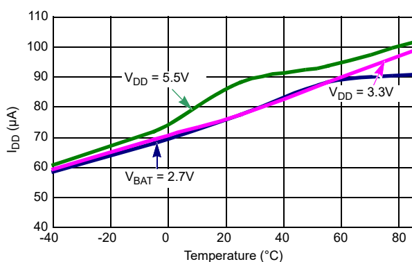
Figure 14. I_{DD} with TSE = 1 vs Temperature
