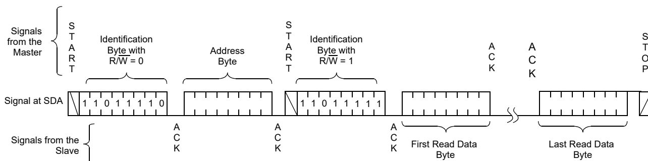
Figure 23. Read Sequence (CSR Slave Address Shown)
