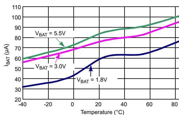
Figure 13. I_{BAT} with TSE = 1, BTSE = 1 vs Temperature
