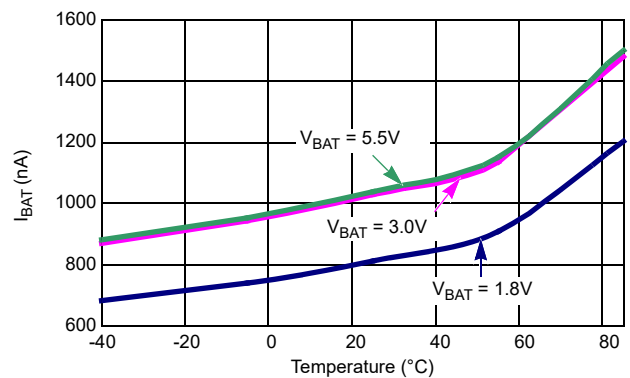
Figure 7. I_{BAT} vs Temperature
